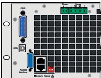
Rear connectors of models with option 3W
