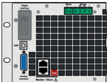
Rear connectors of the standard models
